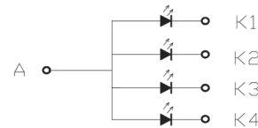
Back Light Circuit
